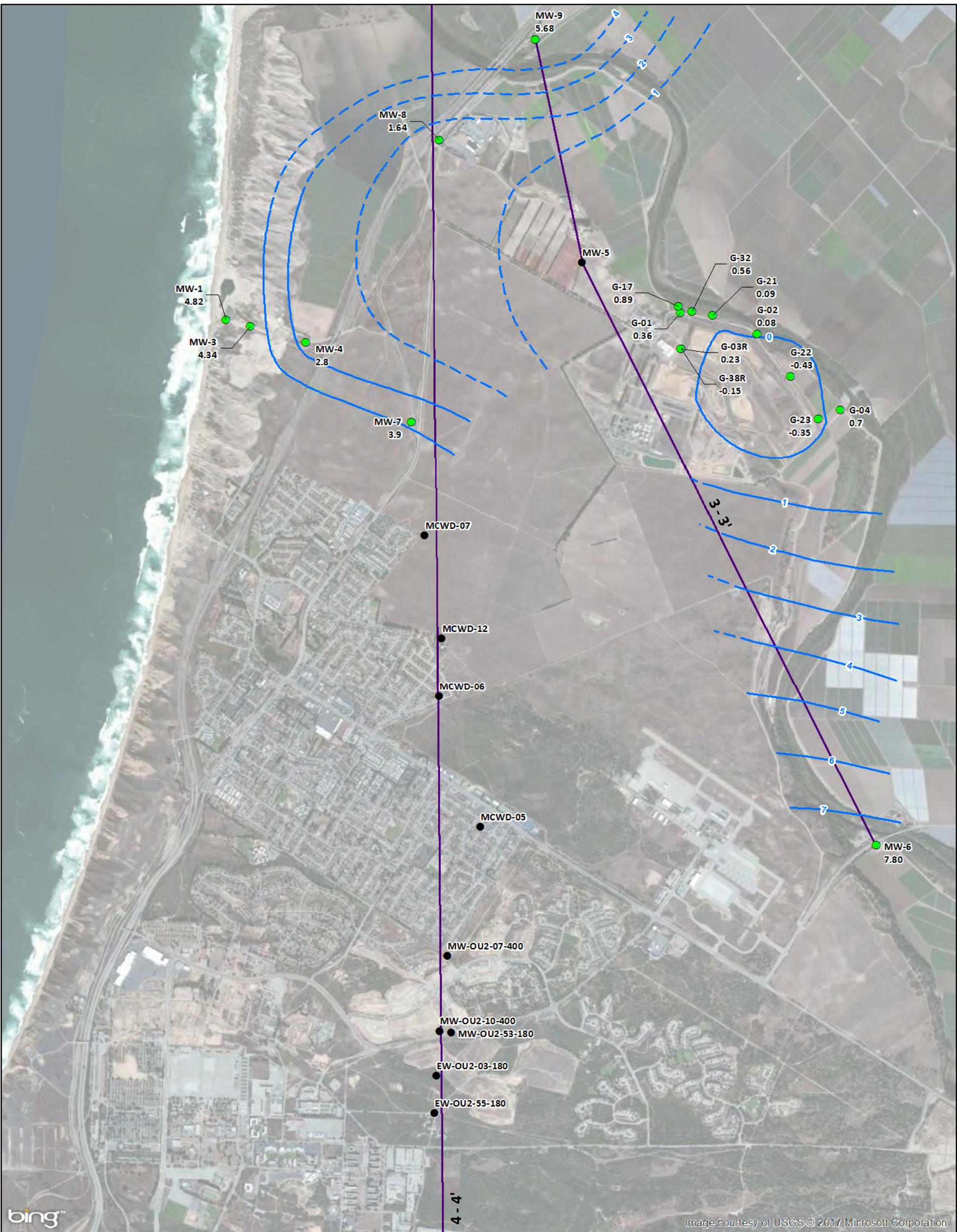
GROUNDWATER ELEVATIONS - "DUNE SAND AQUIFER" (USING MRWMD -2-FOOT AQUIFER WELLS AND MPWSP SHALLOW COMPLECTIONS) FALL 2015
