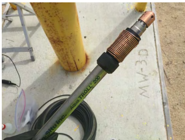
Figure 2-1. Downhole Water Level and Pressure Transducer
