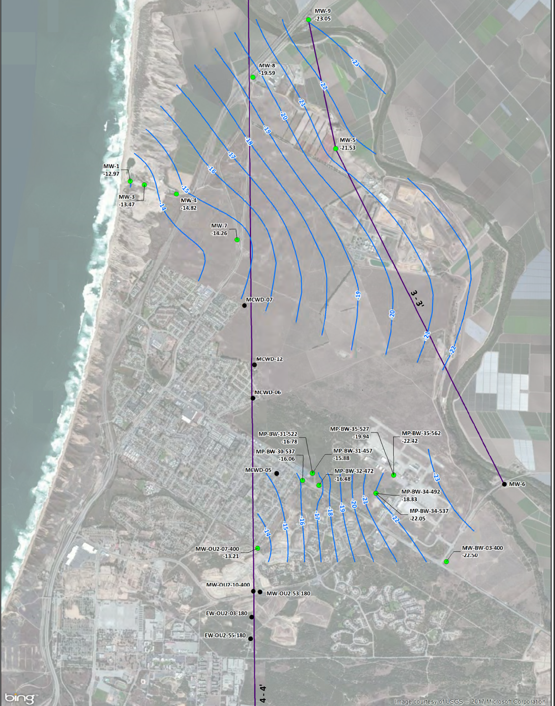
GROUNDWATER ELEVATIONS - "400-FOOT AQUIFER" (USING FORT ORD 400-FOOT AQUIFER WELLS AND MPWSP DEEP COMPLETIONS) FALL 2015
