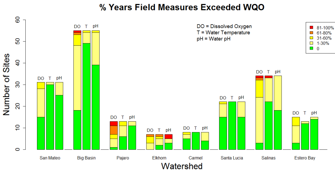
Figure 7: Percentage of years that sites within a watershed exceeded water quality objectives (WQOs) for field measured water chemistry. Only sites monitored ≥5 years were analyzed. The Estrella watershed was omitted because only 1 site was monitored ≥5 years.
