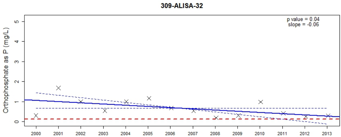
Figure 12. All orthophosphate-P trends observed for Snapshot Day were negative. The three sites with the steepest slopes are shown in this series of plots. Notes the difference in scale on the y-axis. Results below the minimum detection limit are plotted as short vertical dashed lines along the x-axis.
